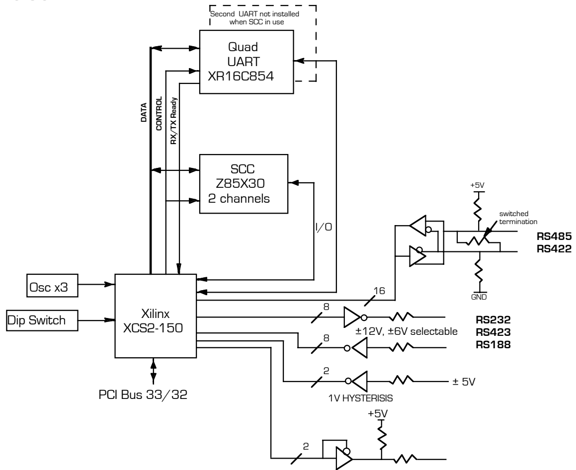
FIGURE 1 PMCSERIAL BLOCK DIAGRAM Other configurations are built into the board layout, including a second quad UART replacing the SCC, and RS-485 I/O. Different oscillators can be installed, or other modifications can be made to accommodate your particular requirements. The new variation will be offered as a "standard" special order product. Please see our web page for current products offered and contact Dynamic Engineering with your custom application.
