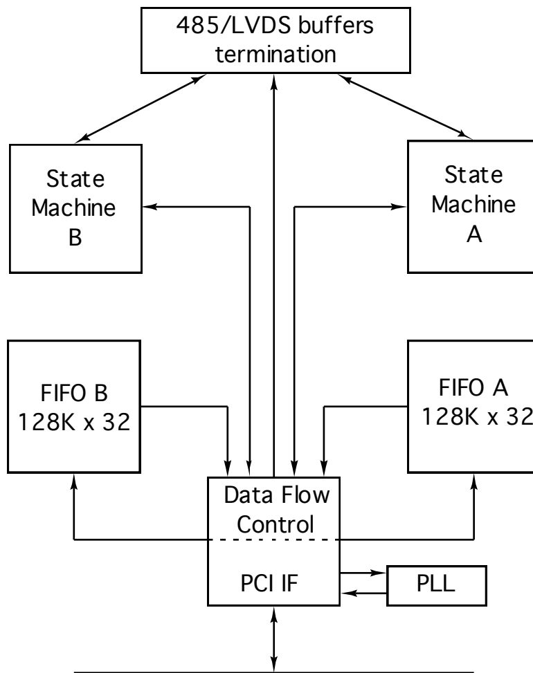
FIGURE 1 PMC-BISERIAL-VI BLOCK DIAGRAM The standard configuration shown in Figure 1 makes use of two external [to the Xilinx ] FIFO's. The external FIFO's are 128K deep x 32 bits wide.
