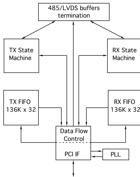
FIGURE 2 PMC-BISERIAL-VI-OSEH BLOCK DIAGRAM
