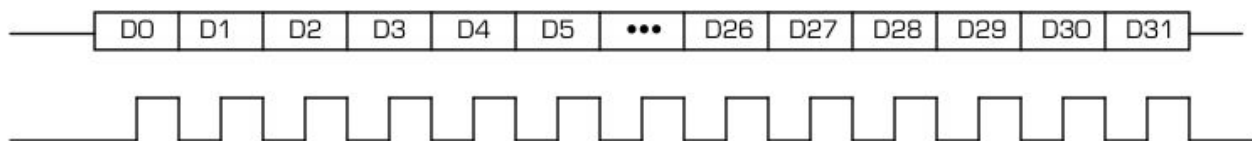
FIGURE 3 PMC BISERIAL-VI-OSEH TIMING DIAGRAM
